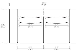
Divano lineare Linear sofa cm 208x104 in 81"8/9x41"
