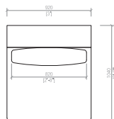
Centrale Central cm 92x104 in 36"2/9x41"
