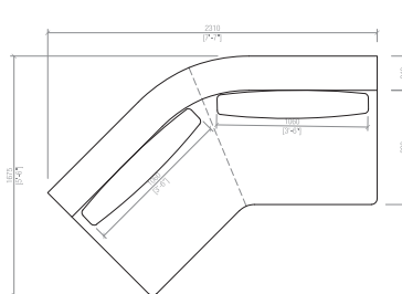
Elemento ad angolo A (dx/sx) Corner element A (L/R) cm 231x167 in 91"x65"3/4
