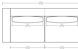
Laterale DX/SX Side R/L cm 232x104 in 91"1/3x41"
