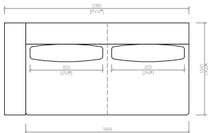
Laterale DX/SX Side R/L cm 208x104 in 81"8/9x41"
