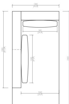
Chaise longue DX/SX Chaise longue R/L cm 128x256 in 50"2/5x100"4/5
