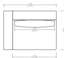
Laterale DX/SX Side R/L cm 140x104 in 55"1/8x41"
