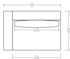
Laterale DX/SX Side R/L cm 152x104 in 59"5/6x41"
