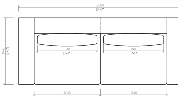
Divano lineare Linear sofa cm 256x104 in 100"4/5x41"
