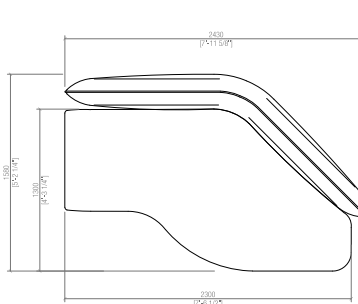
Shaped element with back Elemento sagomato con schienale cm 243x158 in 95"2/3x62"1/5
