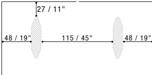
T206B 240X120XH.75 / 94X47XH.30"
