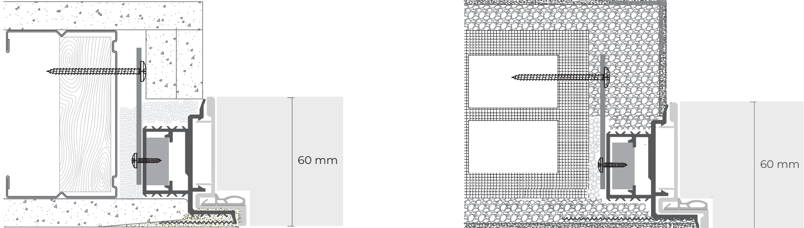
Secret Twin PATENT Complanare a spingere - Flush on the push side
