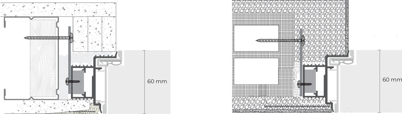
Secret Twin PATENT Complanare a tirare - Flush on the pull side
