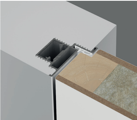
SECRET / flush on the pull side 60 mm
