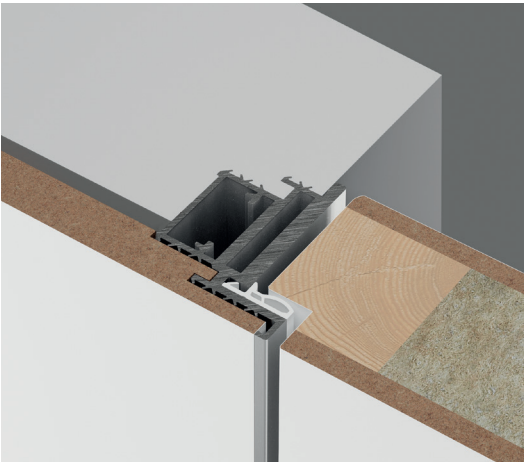
TECNOSECRET / integrated wall paneling, flush on the push side 60 mm
