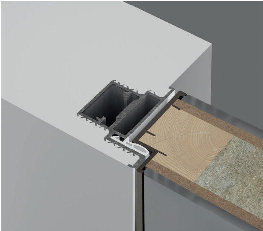
SECRET / flush on the push side 60 mm
