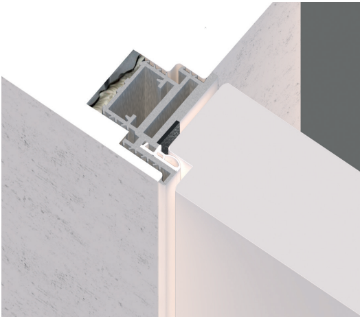
HTB-S4 INVERSO / push side
