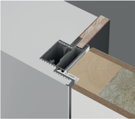
SECRET / with spacer, flush on the push side 60 mm
