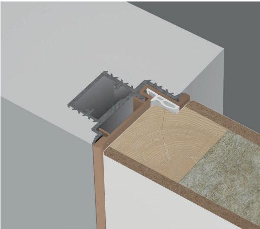
SECRET TWIN / flush on the pull side 60 mm
