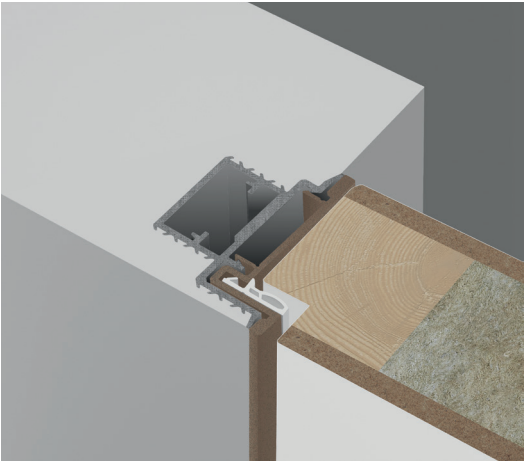
SECRET TWIN / Metal cover, flush on the push side 60 mm
