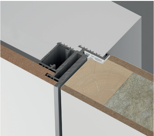
TECNOSECRET / integrated wall paneling, flush on the pull side 60 mm
