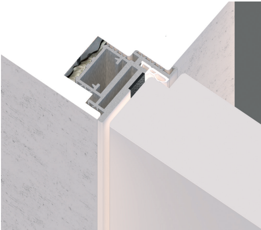
HTB-S4 / pull side
