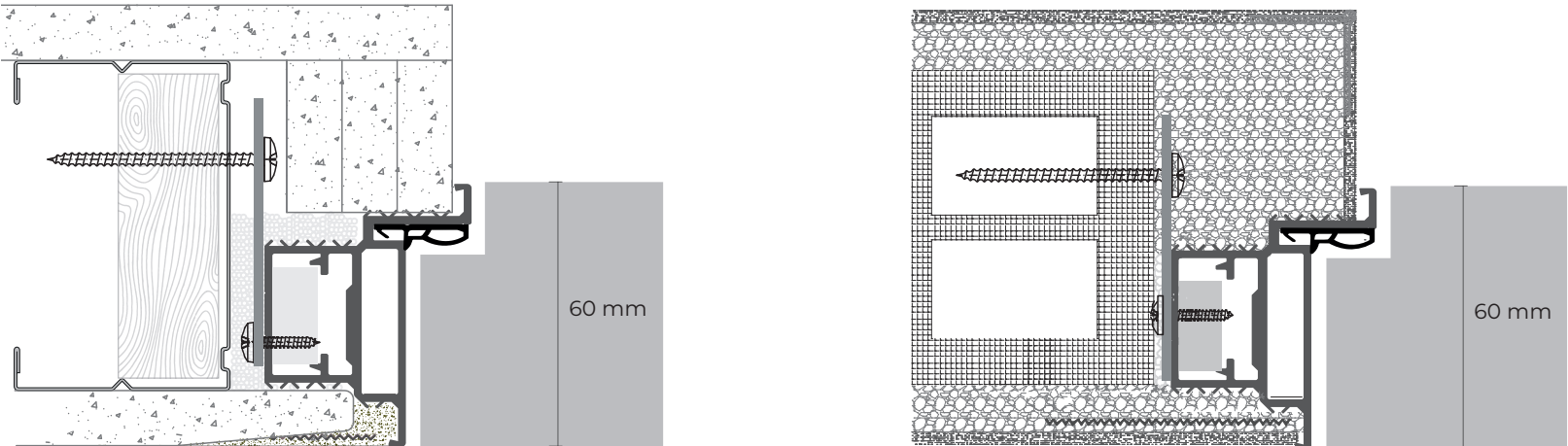
Secret Complanare a tirare - Flush on the pull side
