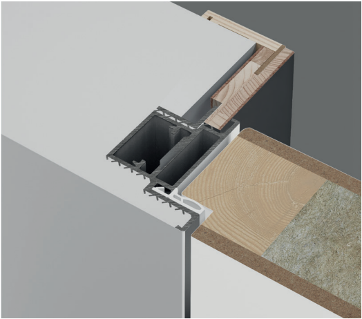
SECRET / with spacer and architraves, flush on the push side 60 mm
