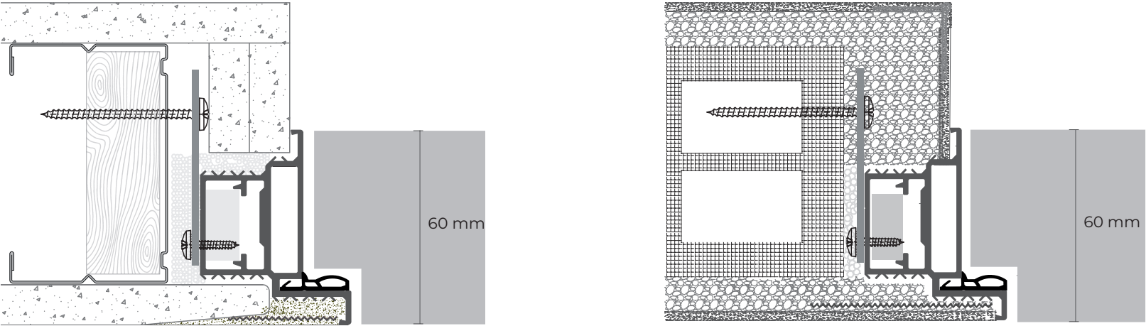
Secret Complanare a spingere - Flush on the push side
