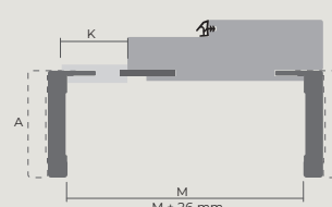
Telaio FN + K a misura Frame FN + K
