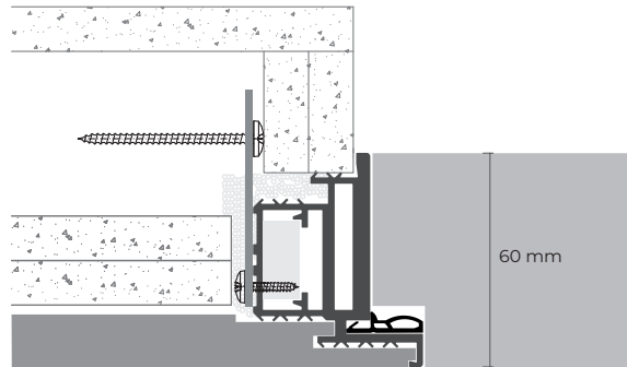
60 mm - a spingere 60 mm - push version
