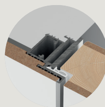
INVERSO 60 INTEGRATED WALL Complanare a spingere Flush on the push side
