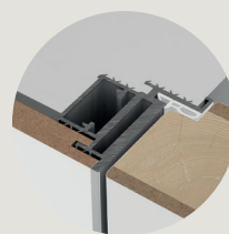
INVERSO 60 INTEGRATED WALL Complanare a tirare Flush on the pull side
