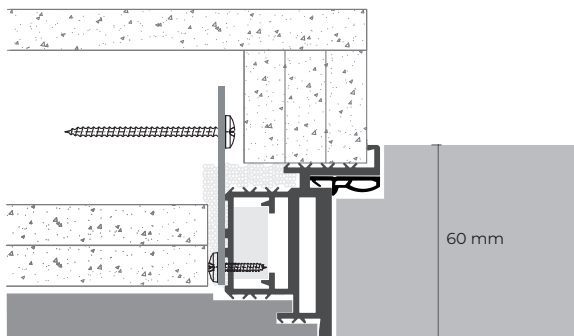
60 mm - a tirare 60 mm - pull version
