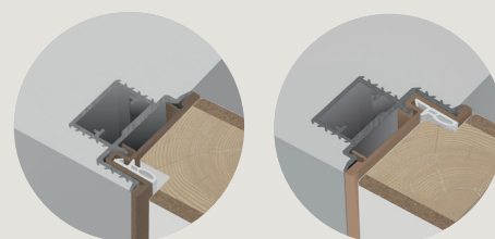
INVERSO 60 Complanare a spingere Flush on the push side INVERSO 60 Complanare a tirare Flush on the pull side
