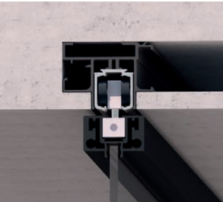
VOLTA 11 / 1 way, 1 rail
