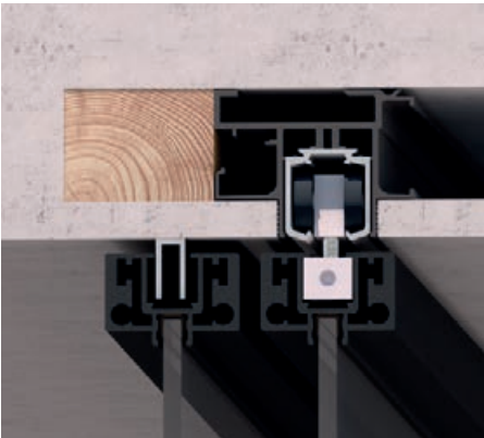
VOLTA 21 / 2 ways, 1 rail
