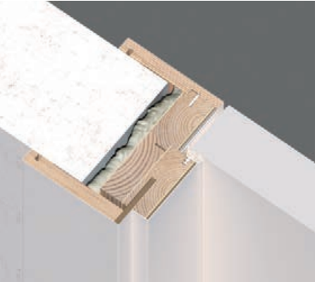
HTB-S3 / push side
