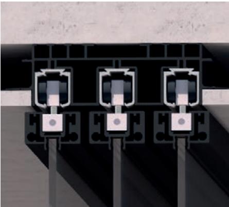
VOLTA 33 / 3 ways, 3 rails
