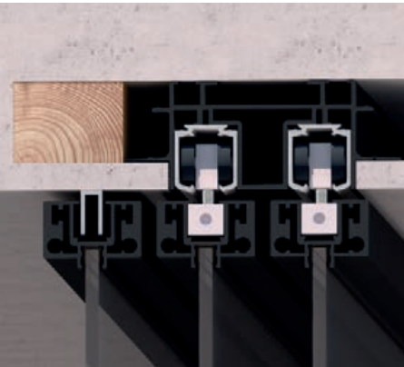
VOLTA 32 / 3 ways, 2 rails
