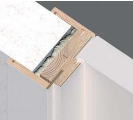
HTB-S9 / push side
