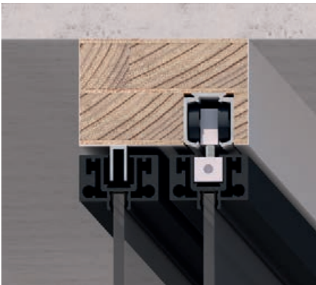
VOLTA M21 / 2 ways, 1 rail
