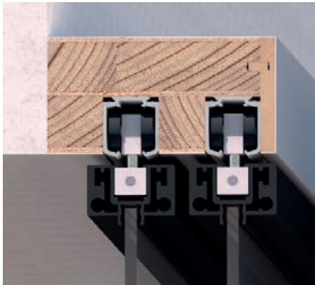
PARI 22 / 2 ways, 2 rails
