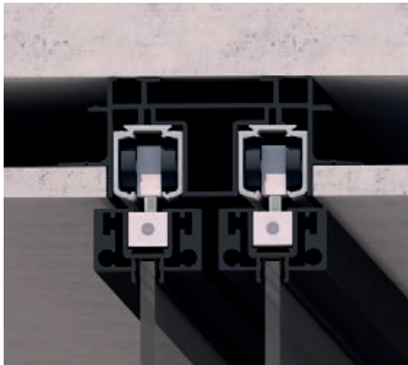
VOLTA 22 / 2 ways, 2 rails
