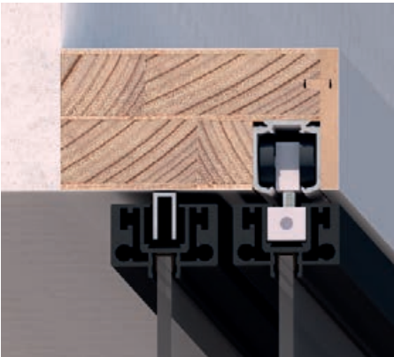
PARI 21 / 2 way, 1 rail
