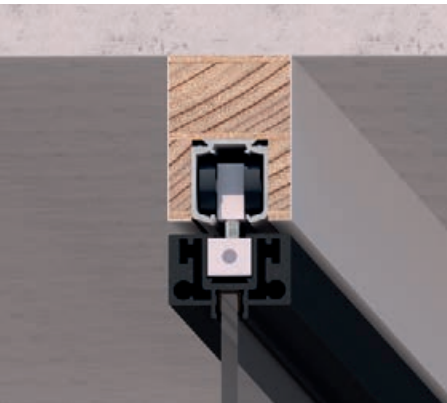
VOLTA M11 / 1 way, 1 rail
